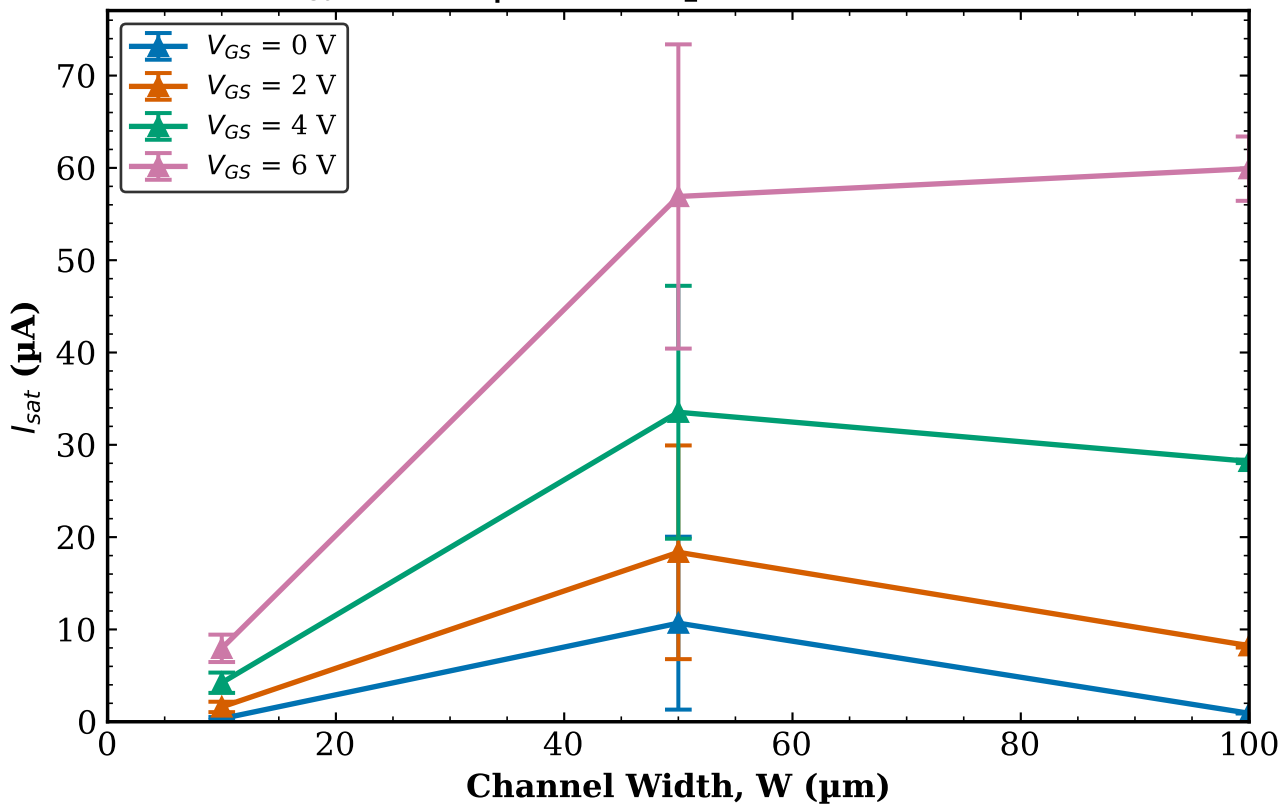
TFT3 Combined (Tr. 1 & 2) I_{sat} vs W | L = 20\text{ }\mu\text{m} (mean \pm std)
